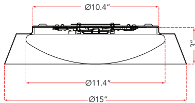
Front Elevation
